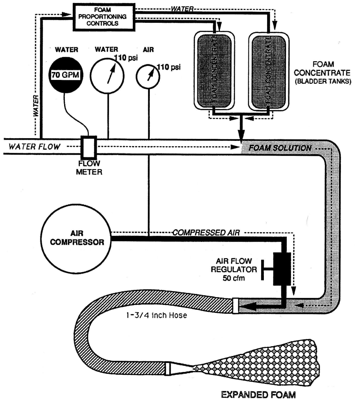
CAFS - System Design & Major Components
